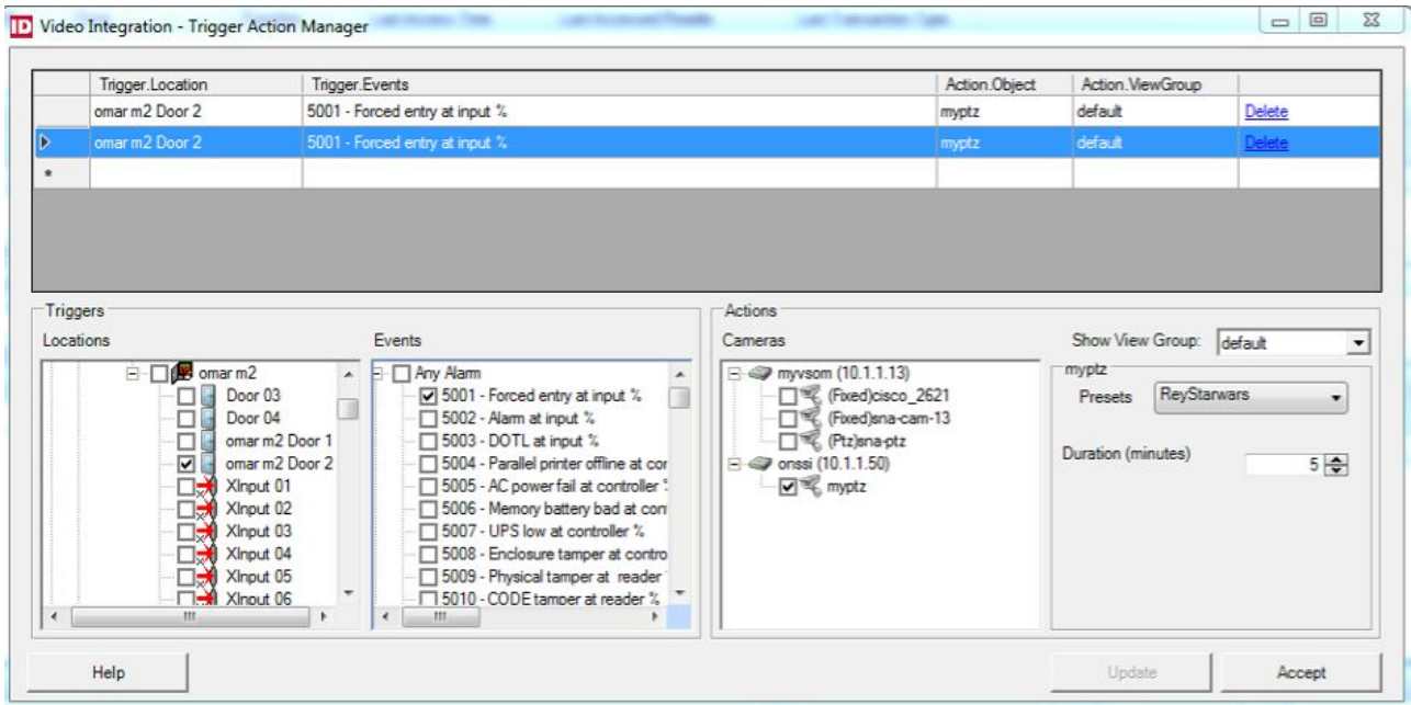
Figure 3: Velocity Trigger Action Manager
